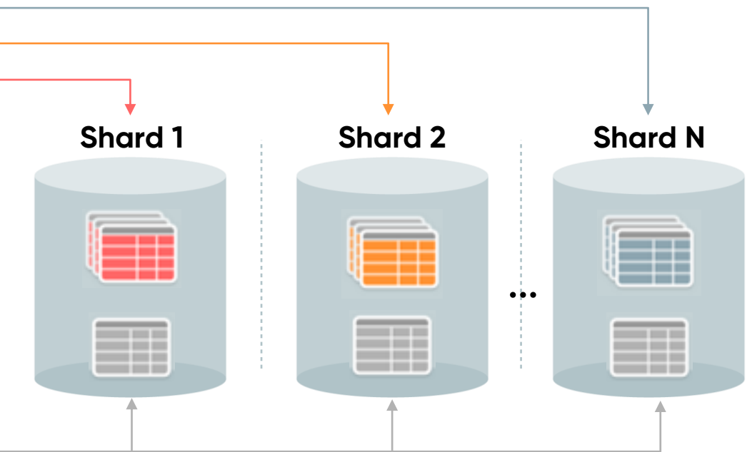
Sharded Tables
